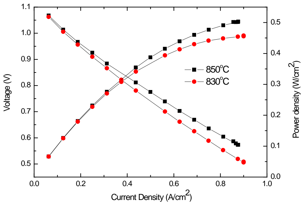
Fig. 7 Electrochemical Performance of 8YSZ Cells
