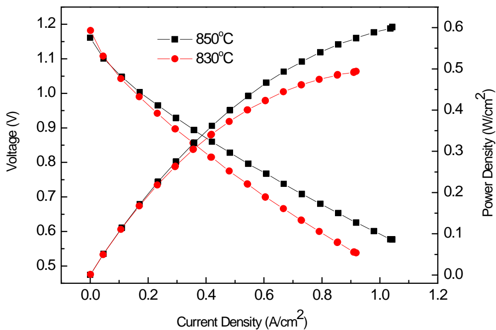
Fig. 8 Electrochemical Performance of SSZ Cells
