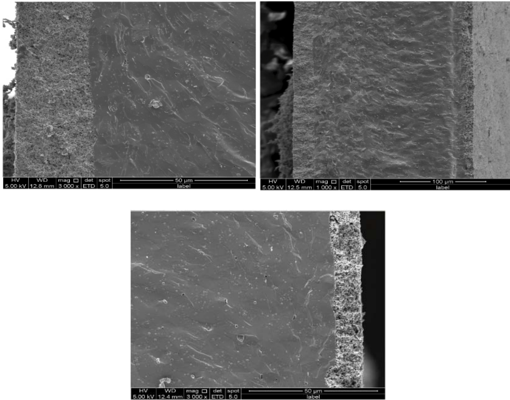
Fig. 4~6 Transverse Cross Section pictures of SSZ Cells
