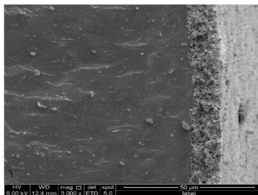
Fig. 1~3 Transverse Cross Section pictures of 8YSZ Cells
